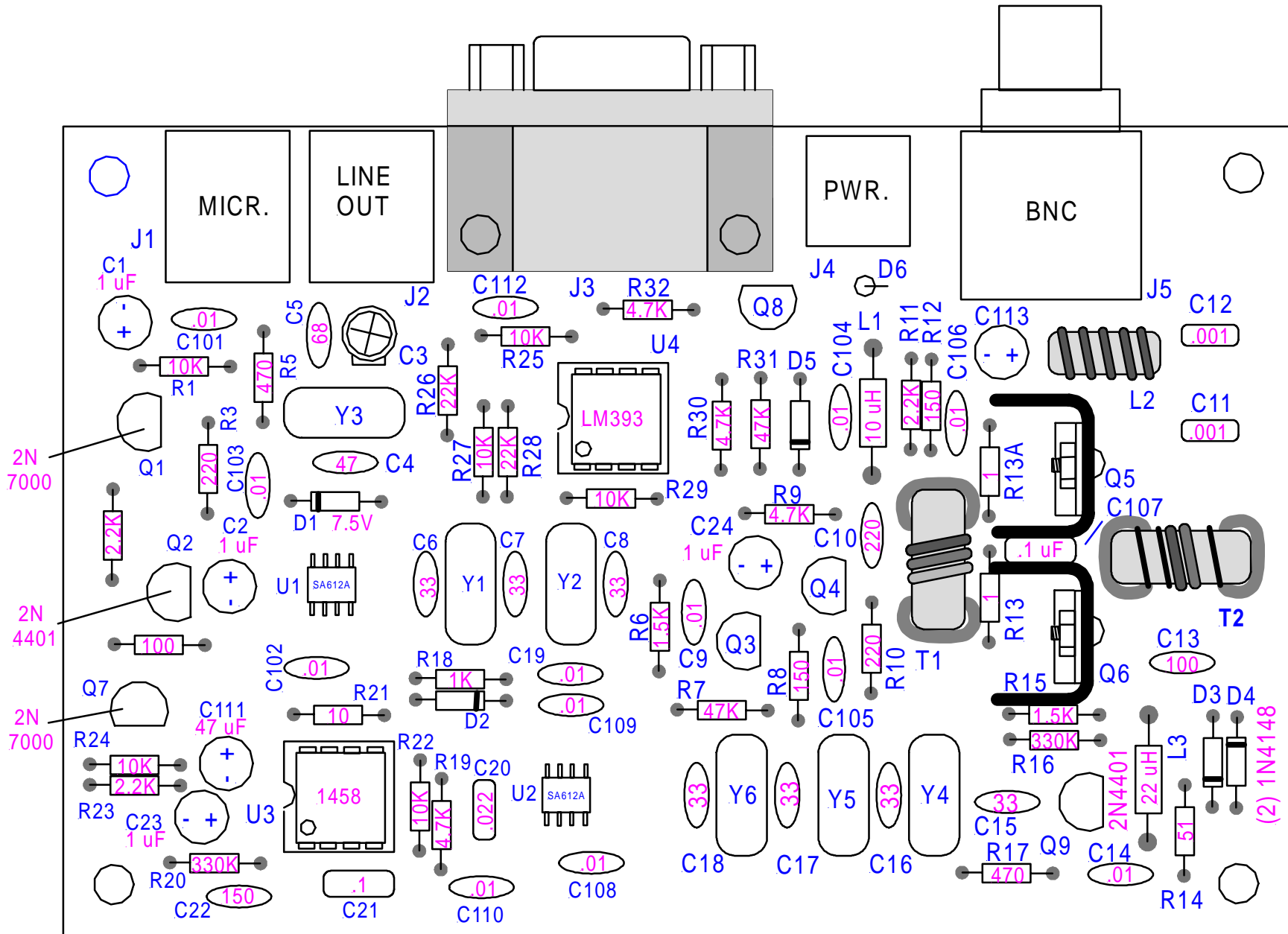
Warbler Board Layout
